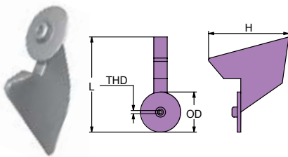
BMW MARK2
