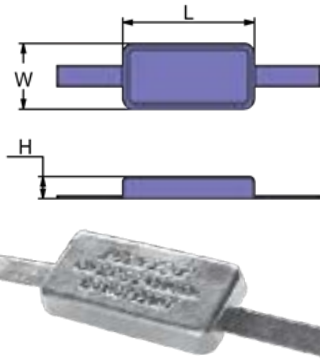
WELD-ON
