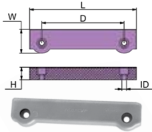
250-270-275-280-285 SERIES
