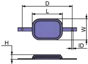
COMBO
