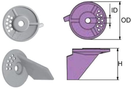
SUZUKI 55-65 HP
