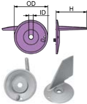
75-85 HP
