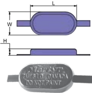
WELD-ON
