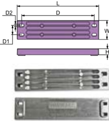
YAMAHA OB ENGINE ANODE 6AW-45251-00
