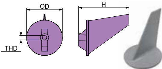
MERCUISER 80 - 140 HP
